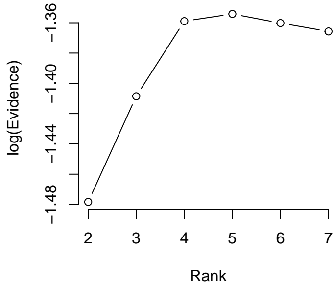
Figure 5: Dependence of log evidence with rank.
