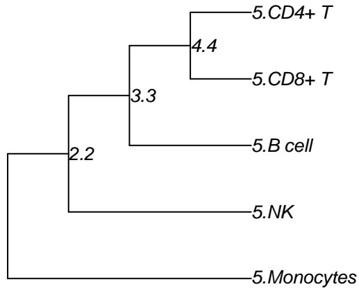
Figure 9: Hierarchical tree of clusters derived from varying ranks. The rank increases from 2 to 5 horizontally and nodes are labeled by cluster IDs which bifurcated in each rank.
