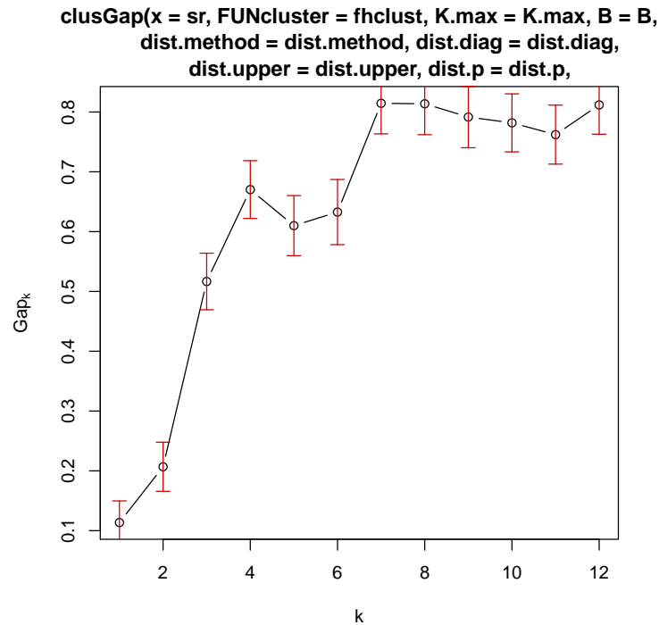
Figure 3: gap statistic plot
