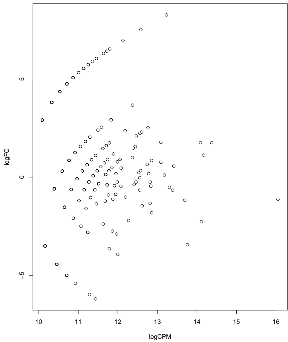
Figure 3: plot(logCPM, logFC)
