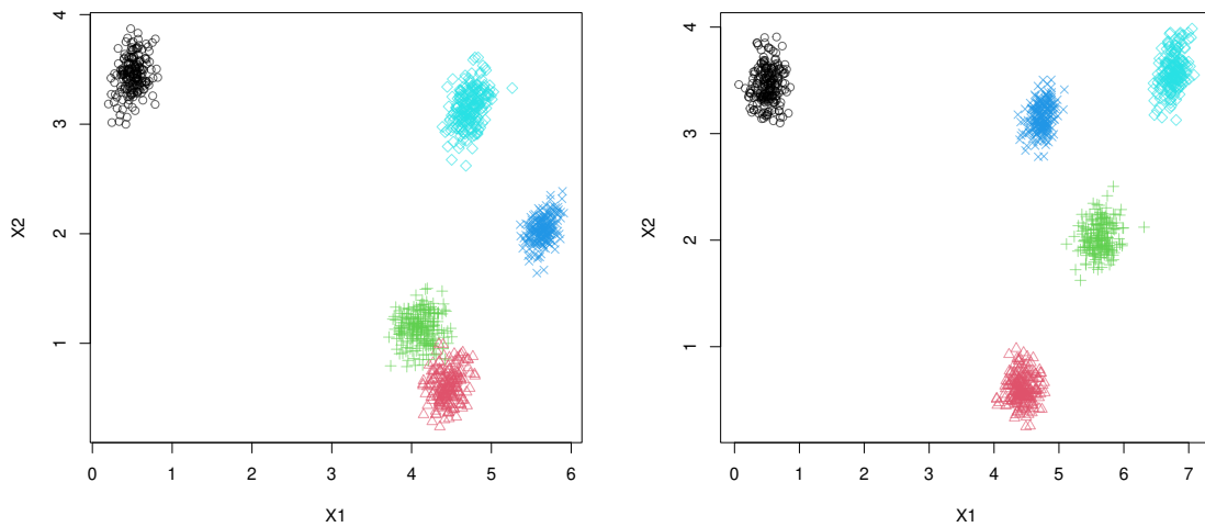
(a) Mahalanobis separation = 3
