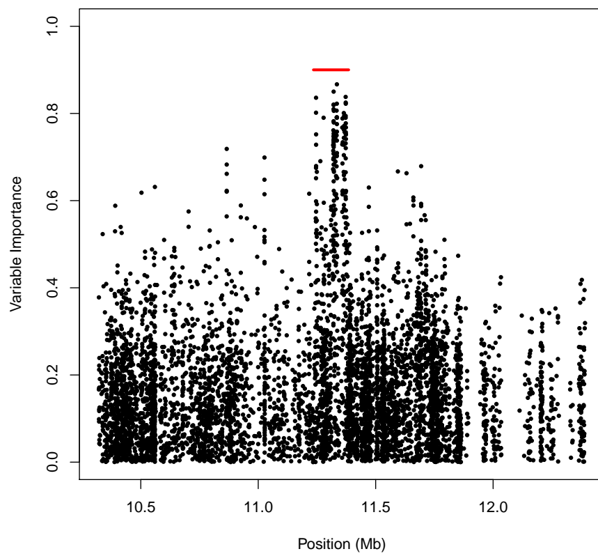
Figure 2: Manhattan-VIMP plot
