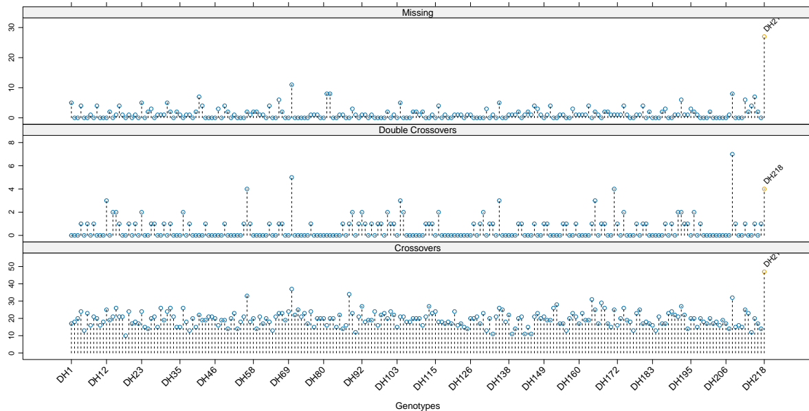
Figure 2.3: Genotype profiles of missing values, double recombinations and recombinations for mapDH.
