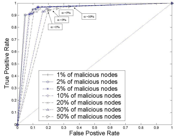
Figure 14: ROC curves.
