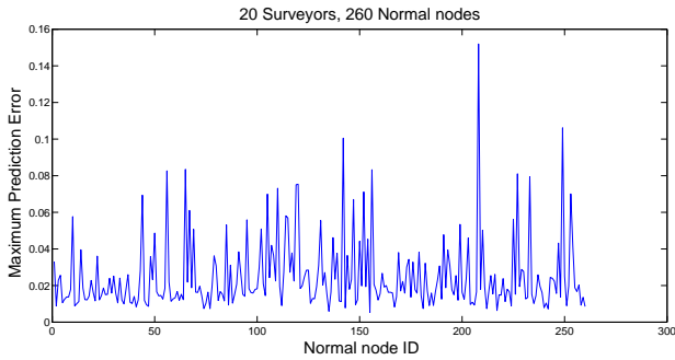
Figure 8: Maximum prediction errors with closest Surveyor.
