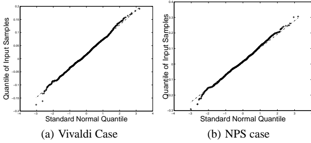
Figure 1: Quantile-Quantile plot of 2 innovation processes.
